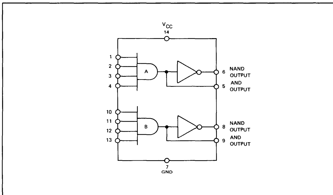
Figure 3-12. Dual Differential Line Driver
