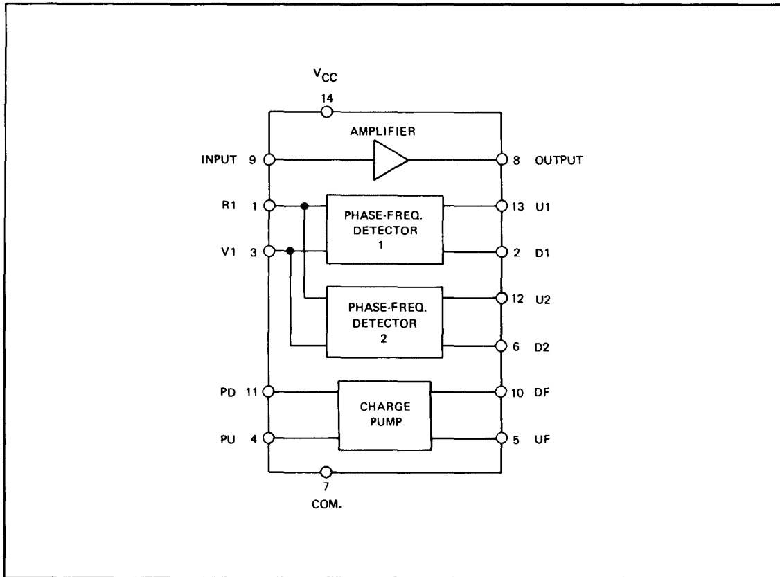
Figure 3-11. Phase-Frequency Detector
