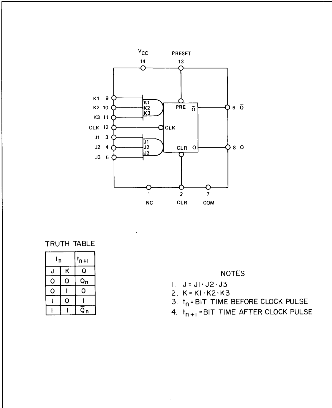
Figure 3-7. J-K Flip-Flop
