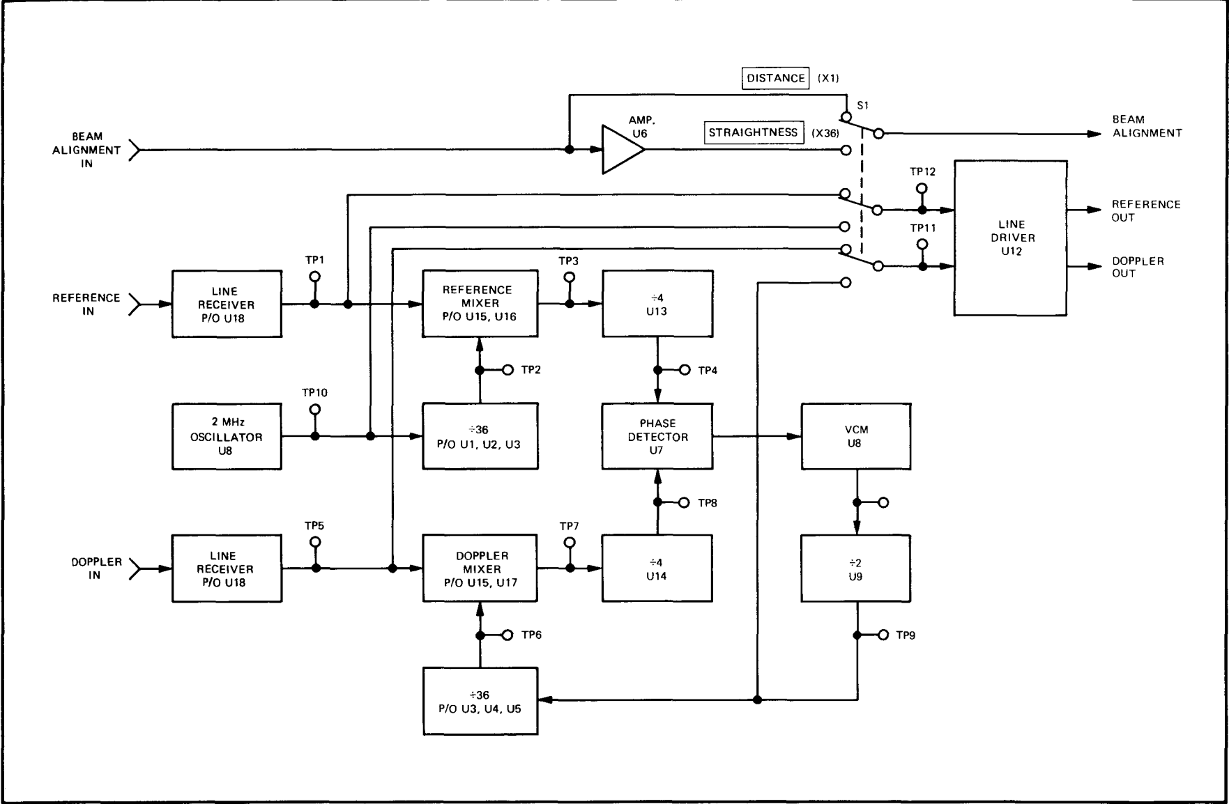
Figure 3-1. Functional Block Diagram of HP 10579-60004 Resolution Extender
