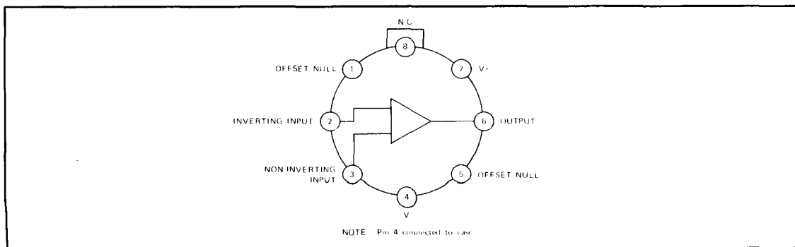
Figure 3-6. Operational Amplifier
